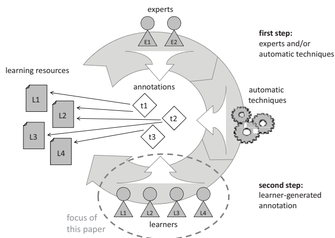
Figure 1: Annotation life-cycle
